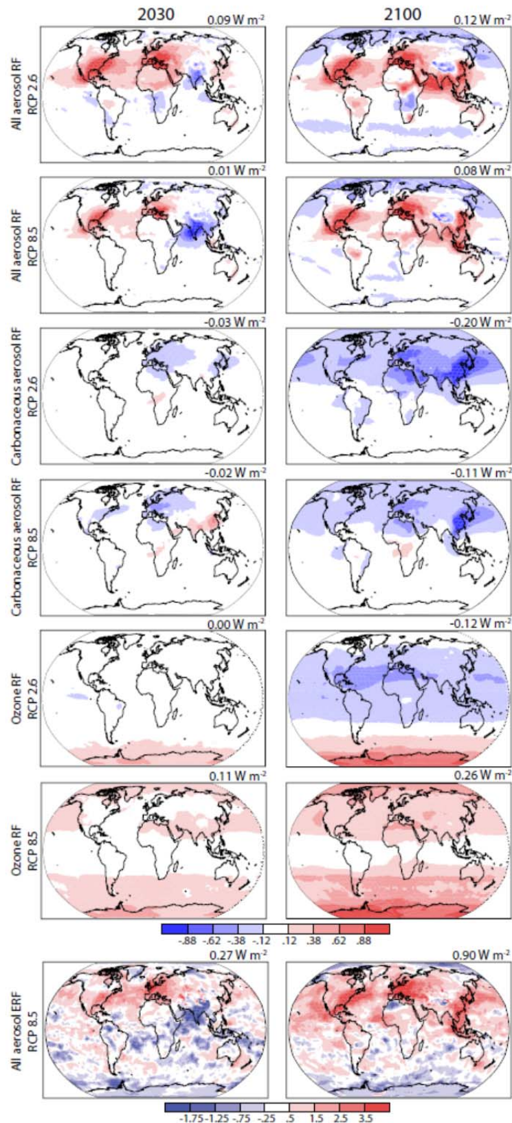
Figure 8.26: Multi-model mean RF ( \text{W m}^{-2} ) due to aerosol-radiation interaction of all anthropogenic aerosols (first and second rows) and anthropogenic carbonaceous (BC+OC) aerosols (third and fourth rows), and total ozone (fifth and sixth rows) in 2030 (left) and 2100 (right) relative to 2000 for RCP2.6 (top each) and RCP8.5 (bottom each) based on the ACCMIP simulations. The seventh row shows multi-model mean ERF ( \text{W m}^{-2} ) by all anthropogenic aerosols in 2030 (left) and 2100 (right) relative to 2000 for RCP8.5. Global area-weighted means are given in the upper right of each panel.
